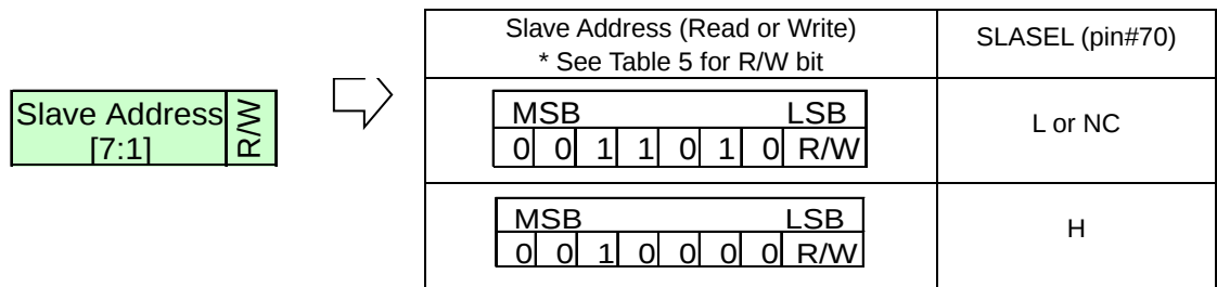
Figure 7 Slave address
