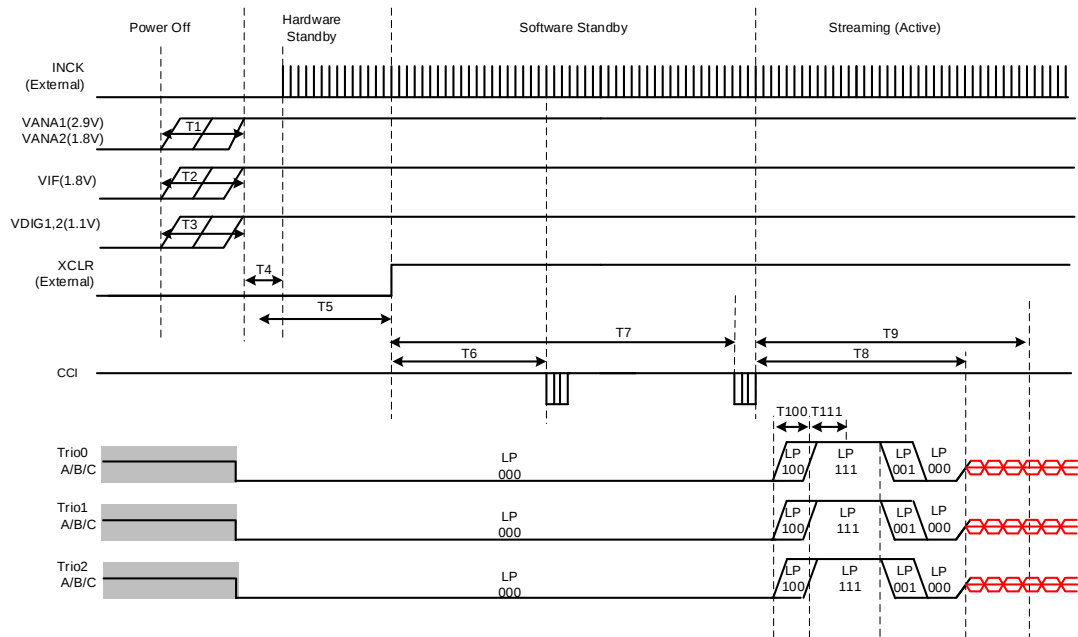
Figure 19 Startup sequence with 2-wire serial communication (C-PHY)
